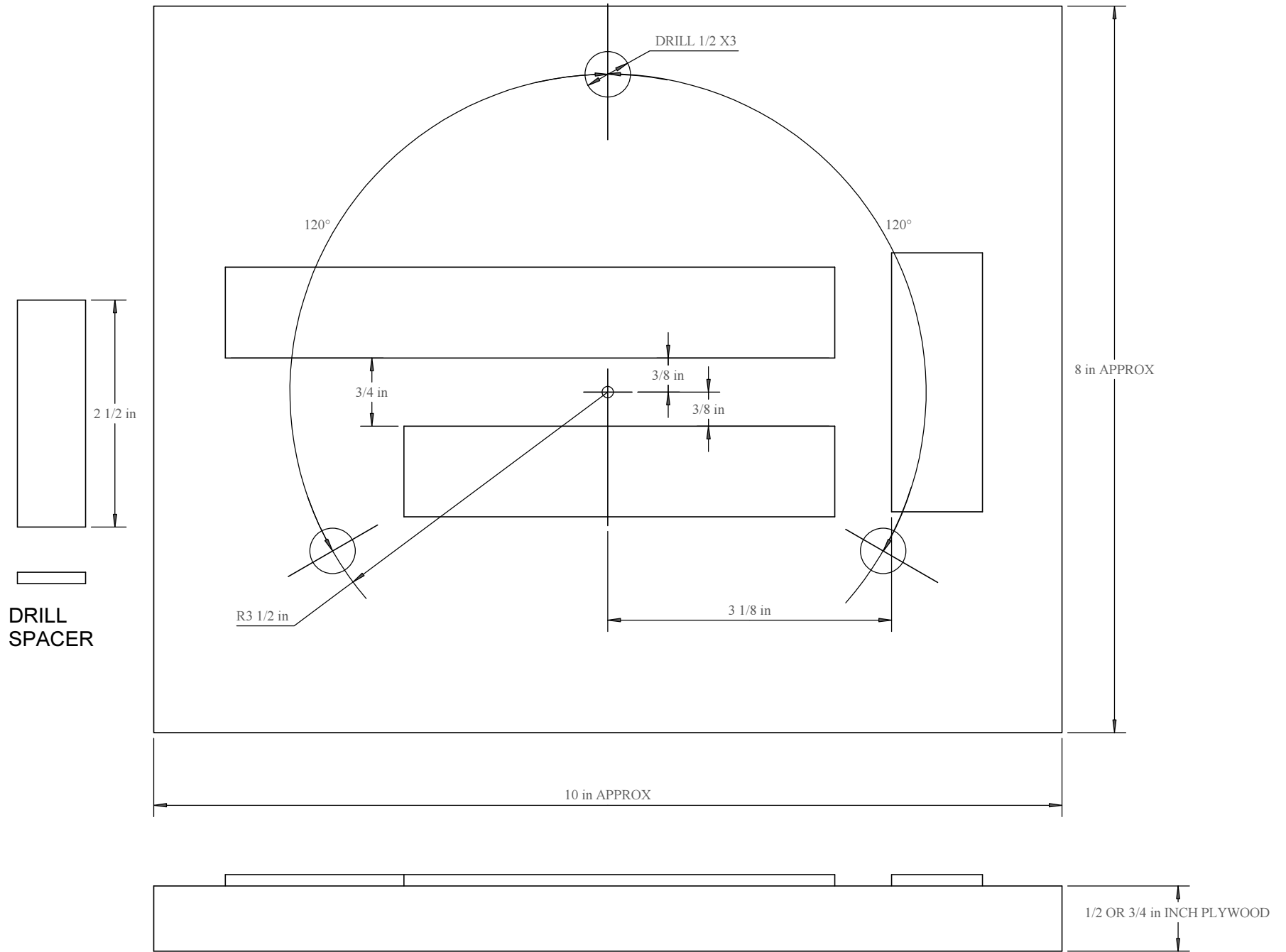
MARKING KNIFE DRILL PRESS JIG
